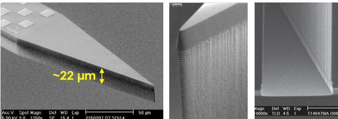
SEM images of the neural probe tip with typical sidewall scallop size <??nm and minimal notching at the Si:SiO 2 interface (Courtesy of imec)
