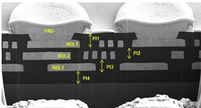
PVD-deposited re-distribution layers (RDL) in FOWLP structure
