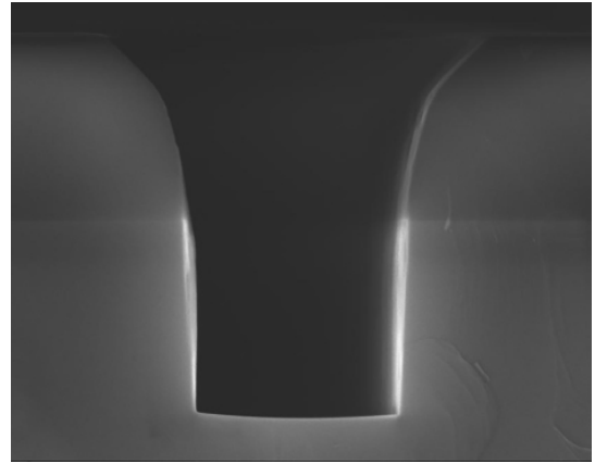
Fig. 4 Power trench with no micro-trenching
