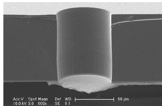
Fig. 1 Backside via etch, 80 \mu\text{m} deep @1.9 \mu\text{m}/\text{min} (Courtesy of ETRI [1] )
